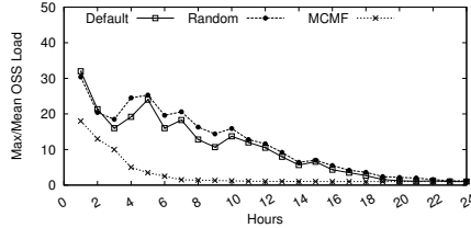
Fig. 12. Max/Mean OSS load over time in simulated setup.
