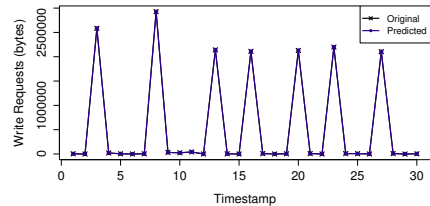
Fig. 8. Orig. vs. predicted requests (Order = 3).
